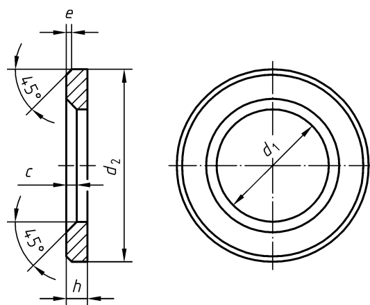
Figure 1 — Dimensions
